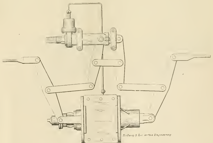
PROPOSED SLACK ADJUSTER ARRANGEMENT FOR PASSENGER BRAKE.
